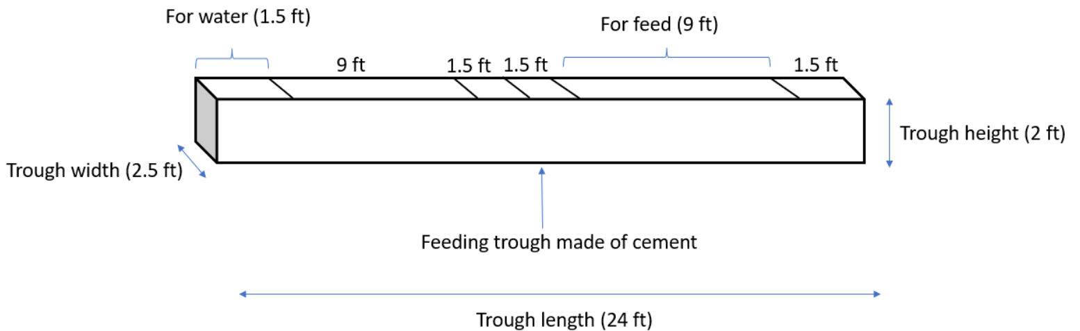
Figure 1: Technical drawing of the technology (improved dairy shed)
