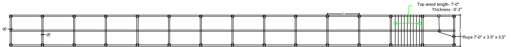
Kundarpara_01 wooden bridge Plan
