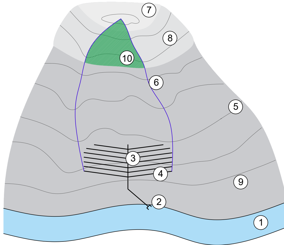
1 - Recipient; 2 - Drainage outlet ; 3 - Conducting drain; 4 - Collecting drain; 5 - Contour line; 6 - Divide of drainage group micro-catchment; 7 - Very permeable soils; 8 - Permeable soils; 9 - Medium and low permeable soils; 10 - Grassing in recharge area
